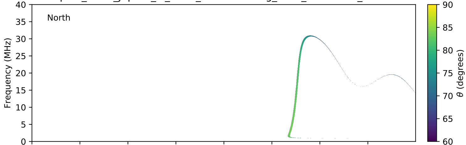
expres_earth_jupiter_io_isaac_lossc-wid1deg_3kev_20150728_v01.cdf
