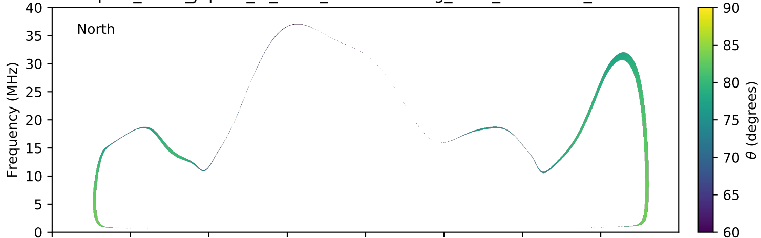
expres_earth_jupiter_io_isaac_lossc-wid1deg_3kev_20150725_v01.cdf
