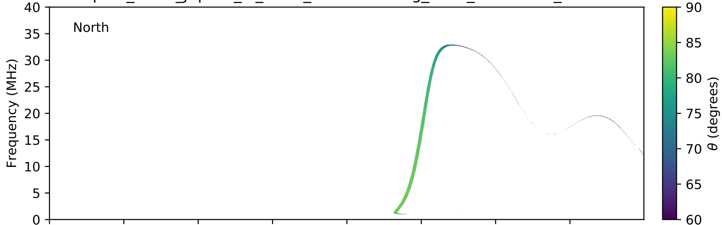
expres_earth_jupiter_io_isaac_lossc-wid1deg_3kev_20150721_v01.cdf
