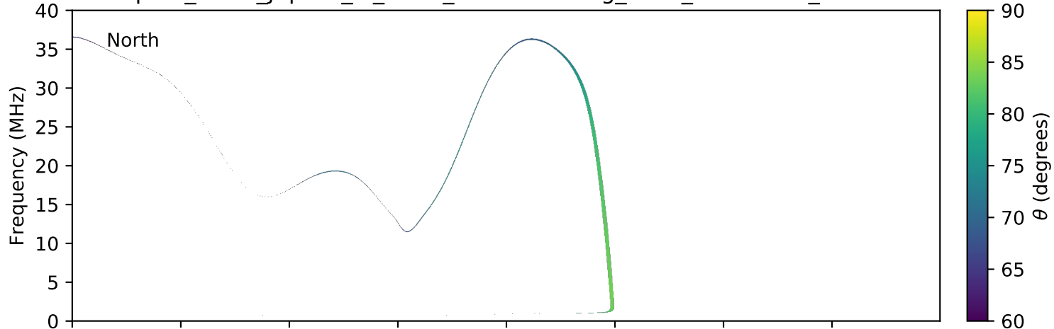
expres_earth_jupiter_io_isaac_lossc-wid1deg_3kev_20150720_v01.cdf
