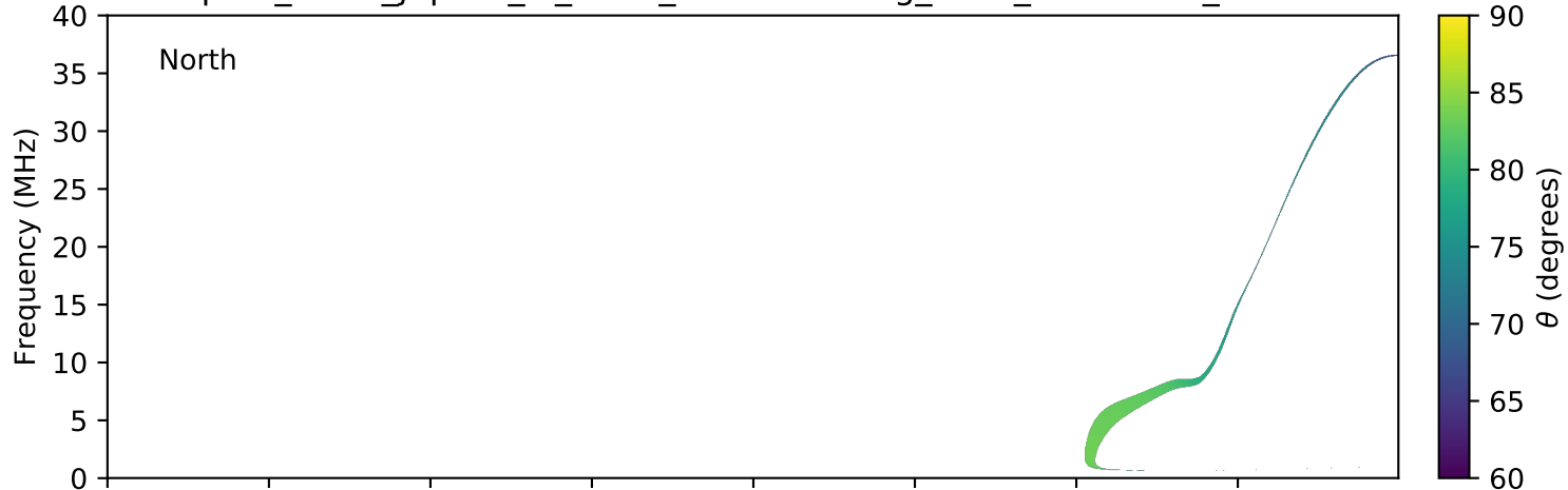
expres_earth_jupiter_io_isaac_lossc-wid1deg_3kev_20150719_v01.cdf
