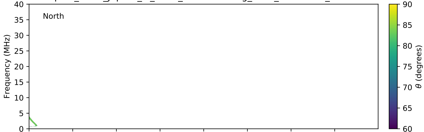
expres_earth_jupiter_io_isaac_lossc-wid1deg_3kev_20150717_v01.cdf
