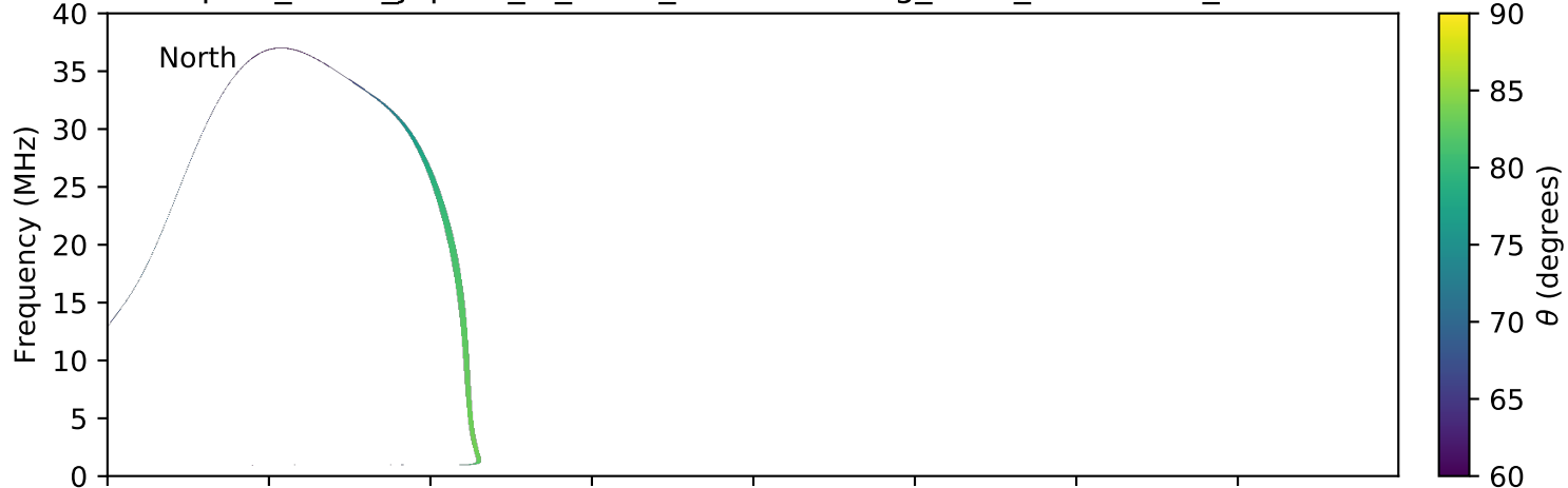
expres_earth_jupiter_io_isaac_lossc-wid1deg_3kev_20150715_v01.cdf
