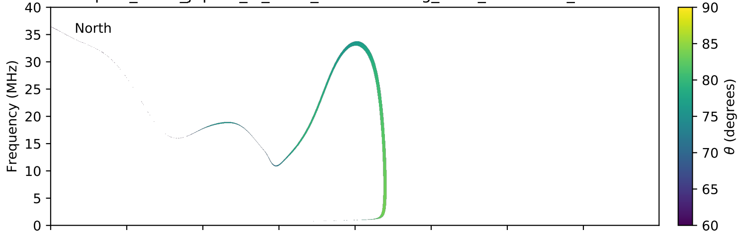
expres_earth_jupiter_io_isaac_lossc-wid1deg_3kev_20150713_v01.cdf
