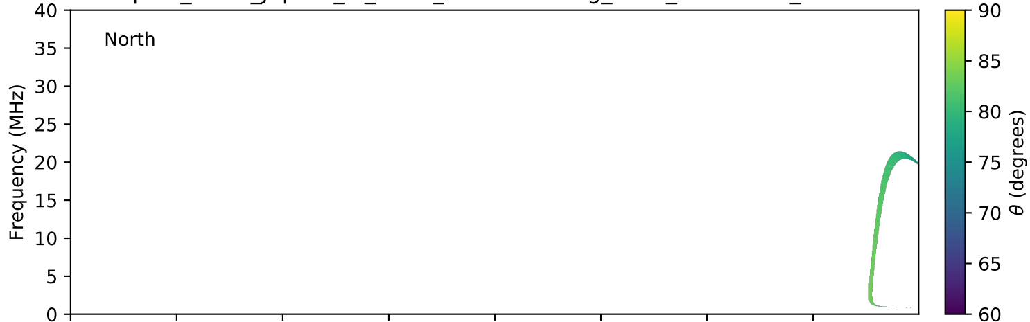
expres_earth_jupiter_io_isaac_lossc-wid1deg_3kev_20150710_v01.cdf
