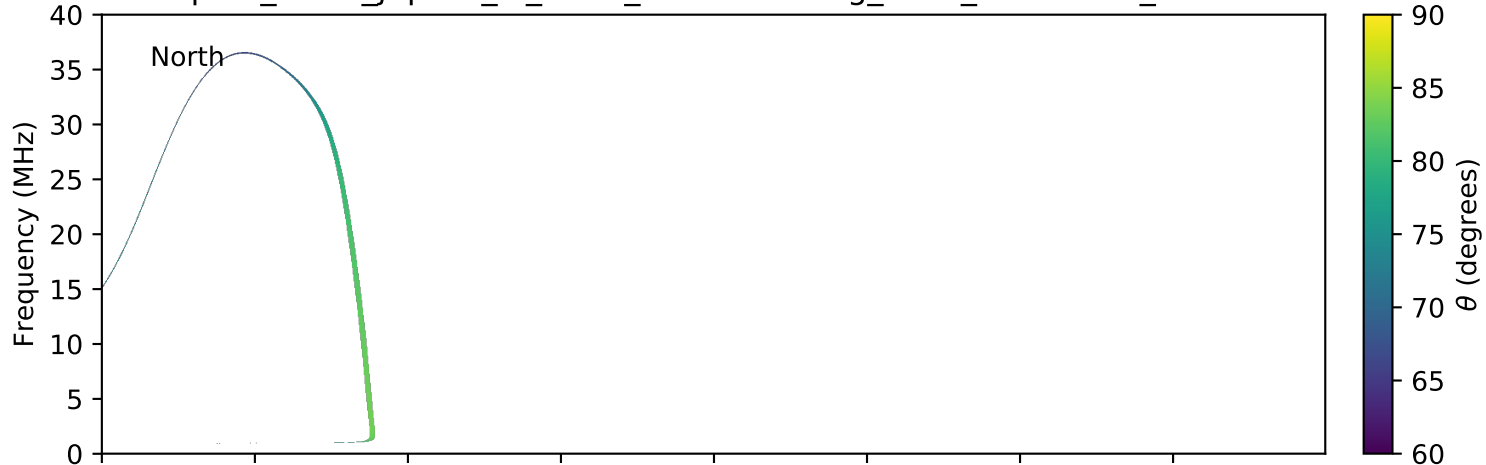
expres_earth_jupiter_io_isaac_lossc-wid1deg_3kev_20150708_v01.cdf
