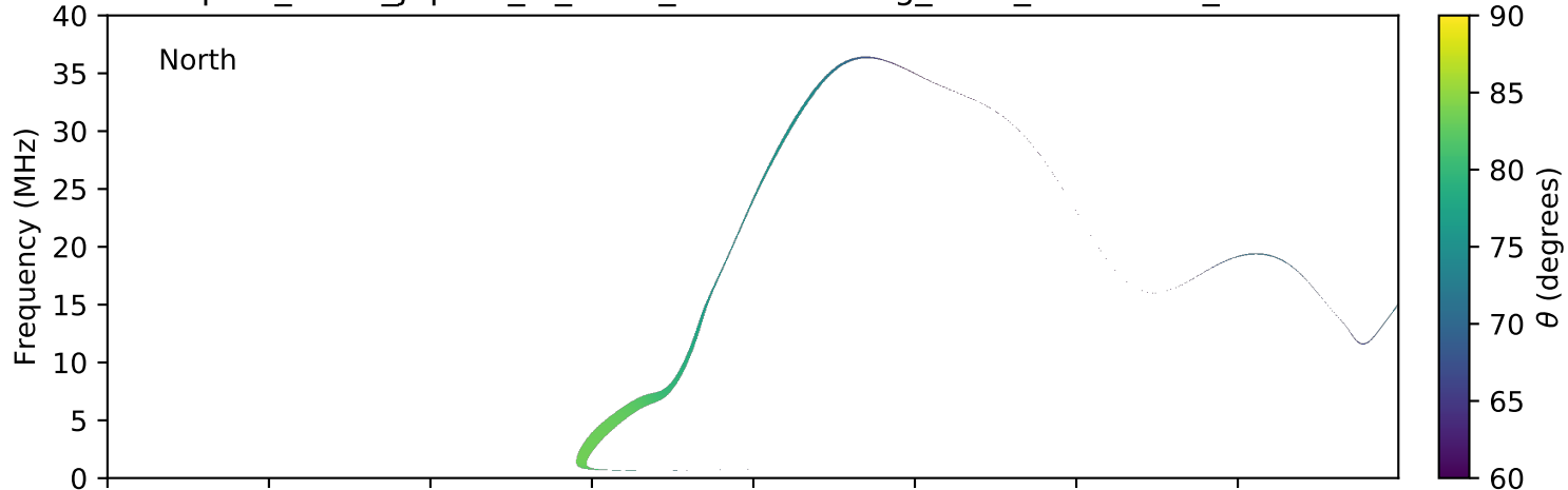
expres_earth_jupiter_io_isaac_lossc-wid1deg_3kev_20150707_v01.cdf
