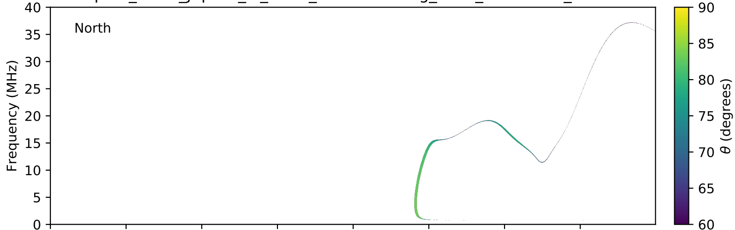
expres_earth_jupiter_io_isaac_lossc-wid1deg_3kev_20150705_v01.cdf
