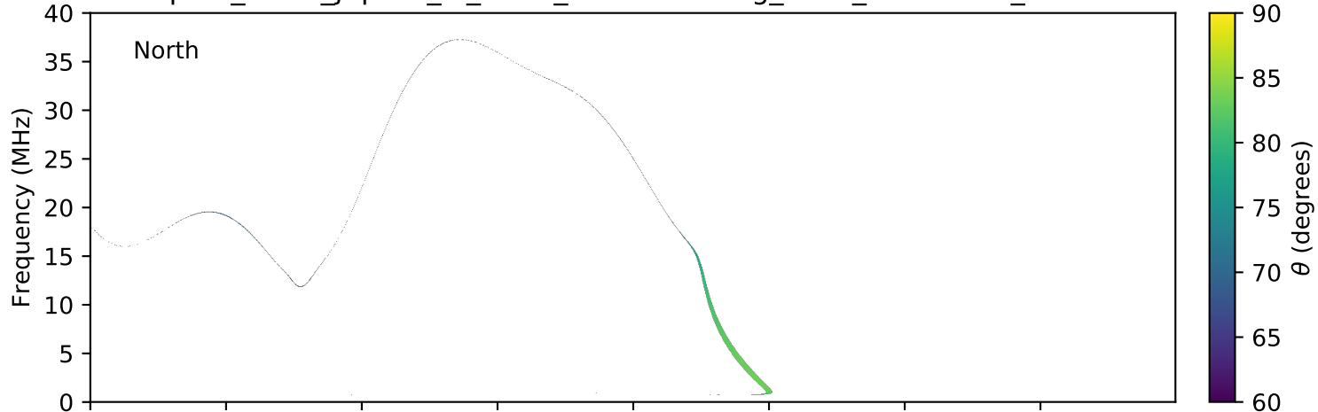
expres_earth_jupiter_io_isaac_lossc-wid1deg_3kev_20150704_v01.cdf
