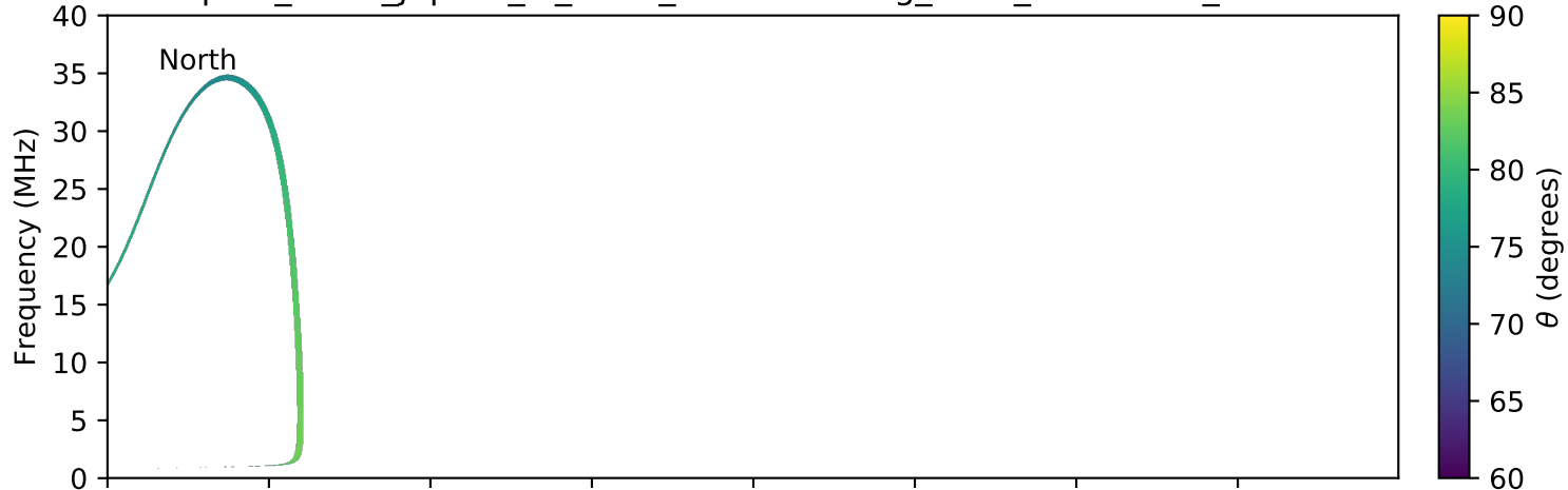
expres_earth_jupiter_io_isaac_lossc-wid1deg_3kev_20150701_v01.cdf
