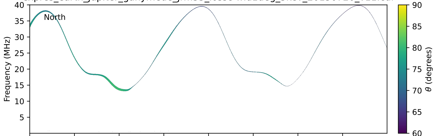
expres_earth_jupiter_ganymede_jrm33_lossc-wid1deg_3kev_20150720_v11.cdf
