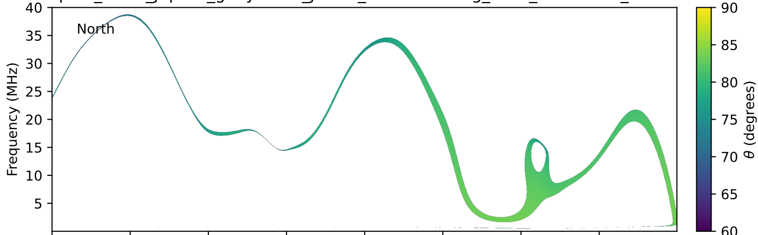
expres_earth_jupiter_ganymede_jrm33_lossc-wid1deg_3kev_20150701_v11.cdf
