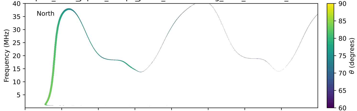
expres_earth_jupiter_europa_jrm33_lossc-wid1deg_3kev_20150705_v11.cdf
