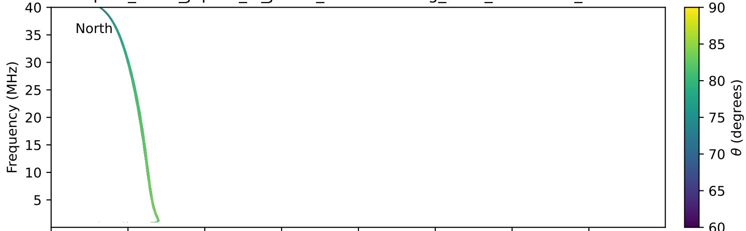
expres_earth_jupiter_io_jrm33_lossc-wid1deg_3kev_20150629_v11.cdf
