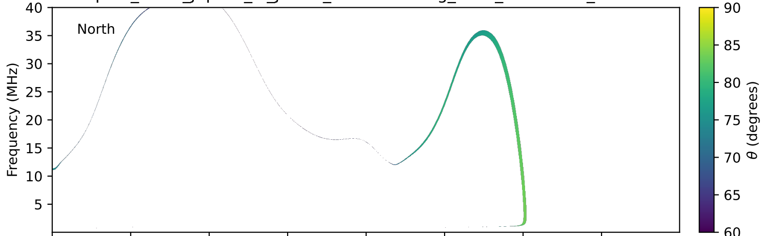
expres_earth_jupiter_io_jrm33_lossc-wid1deg_3kev_20150618_v11.cdf
