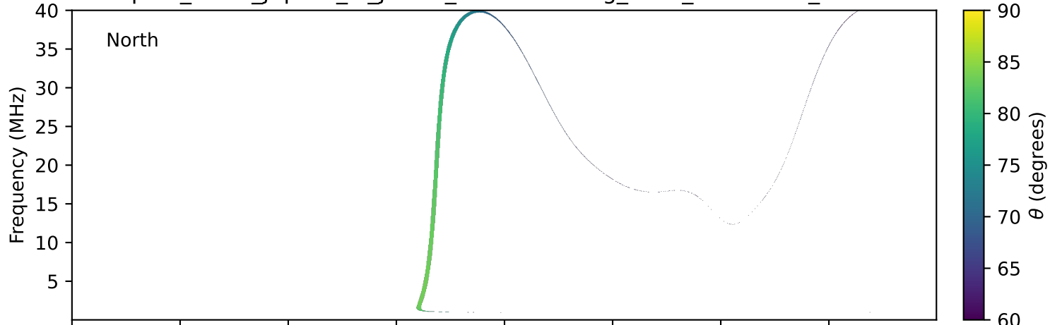
expres_earth_jupiter_io_jrm33_lossc-wid1deg_3kev_20150614_v11.cdf
