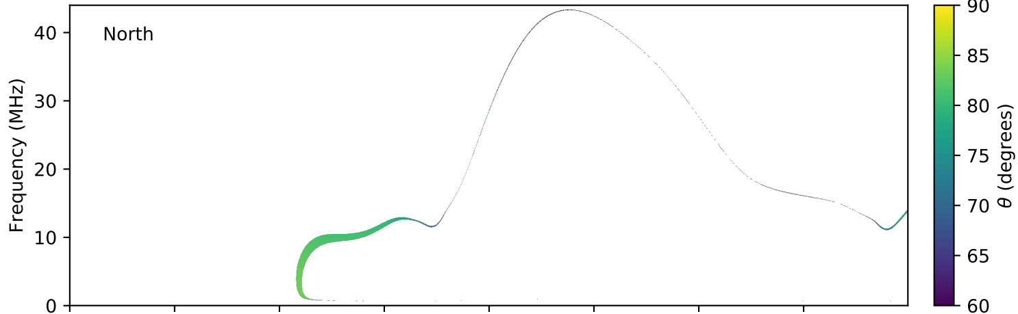
expres_earth_jupiter_io_jrm09_lossc-wid1deg_3kev_20150630_v01.cdf
