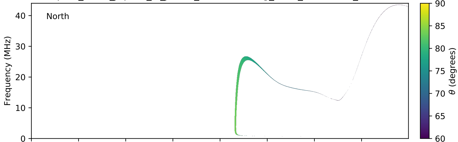
expres_earth_jupiter_io_jrm09_lossc-wid1deg_3kev_20150628_v01.cdf
