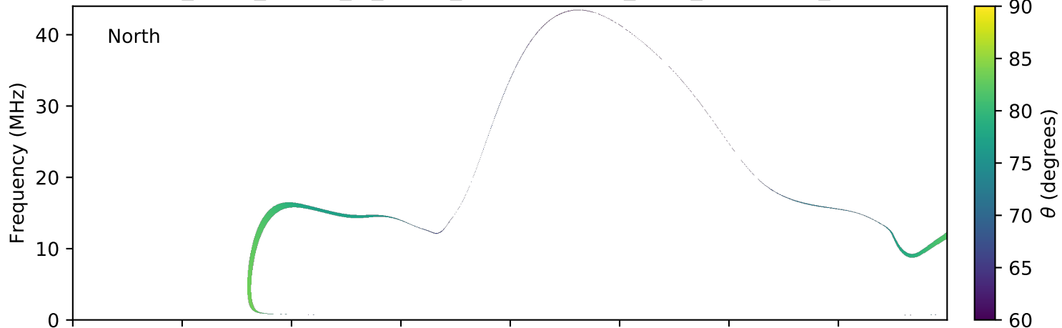
expres_earth_jupiter_io_jrm09_lossc-wid1deg_3kev_20150623_v01.cdf
