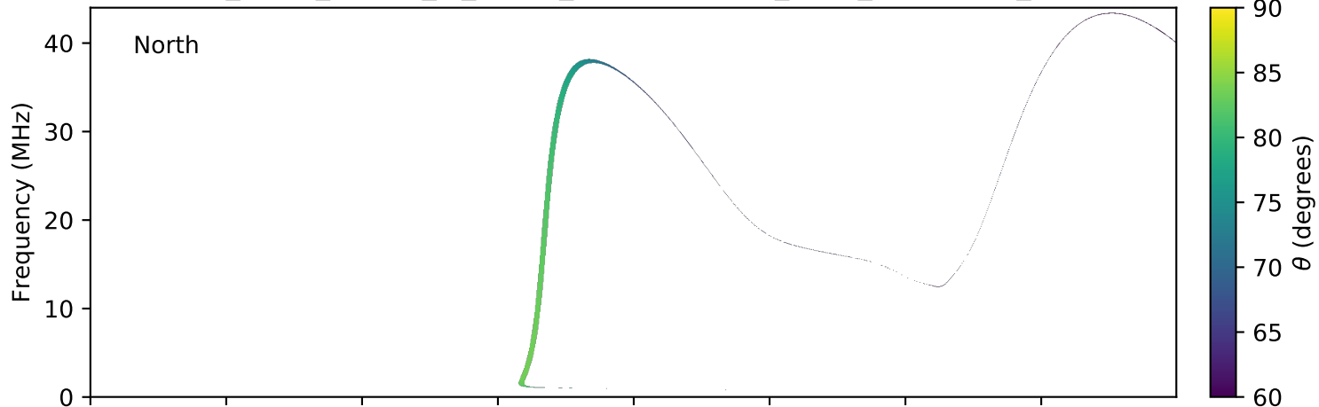
expres_earth_jupiter_io_jrm09_lossc-wid1deg_3kev_20150614_v01.cdf
