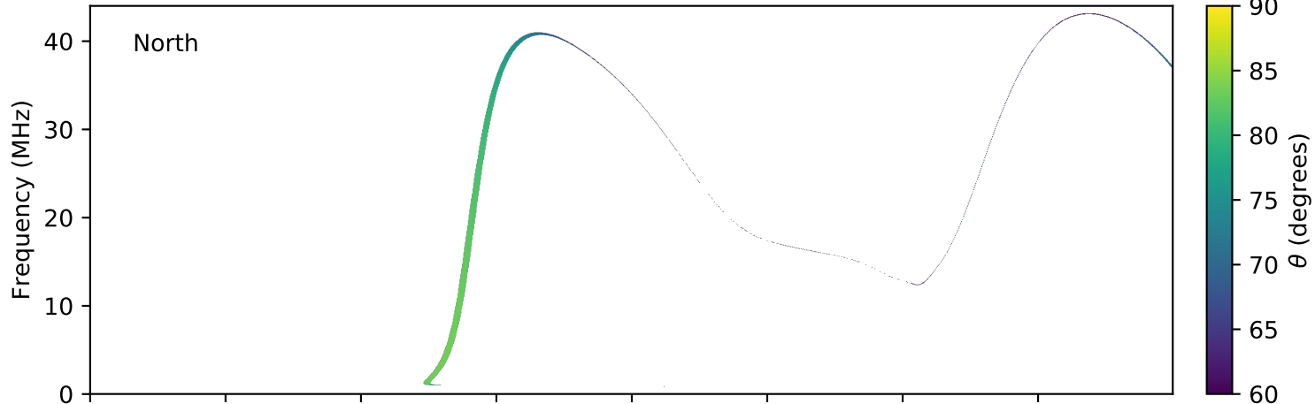
expres_earth_jupiter_io_jrm09_lossc-wid1deg_3kev_20150607_v01.cdf
