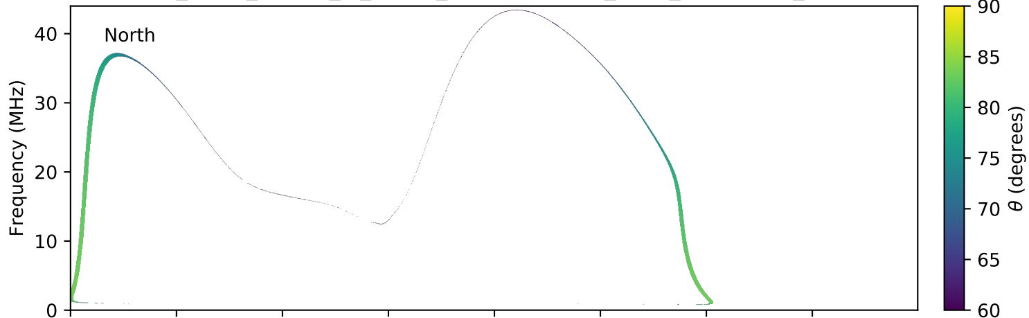
expres_earth_jupiter_io_jrm09_lossc-wid1deg_3kev_20150602_v01.cdf
