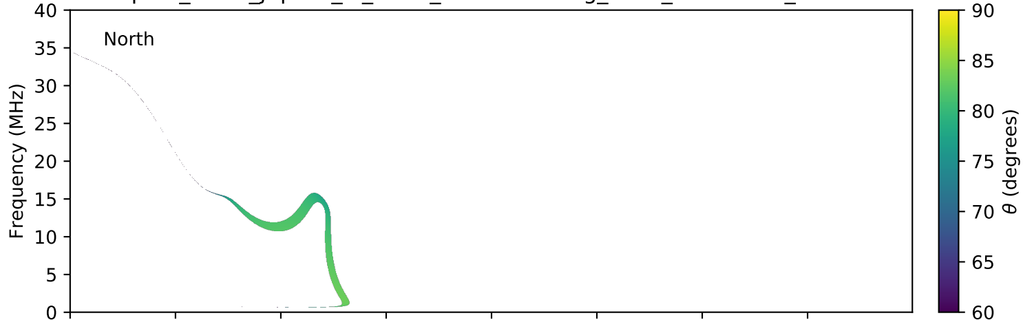
expres_earth_jupiter_io_isaac_lossc-wid1deg_3kev_20150629_v01.cdf
