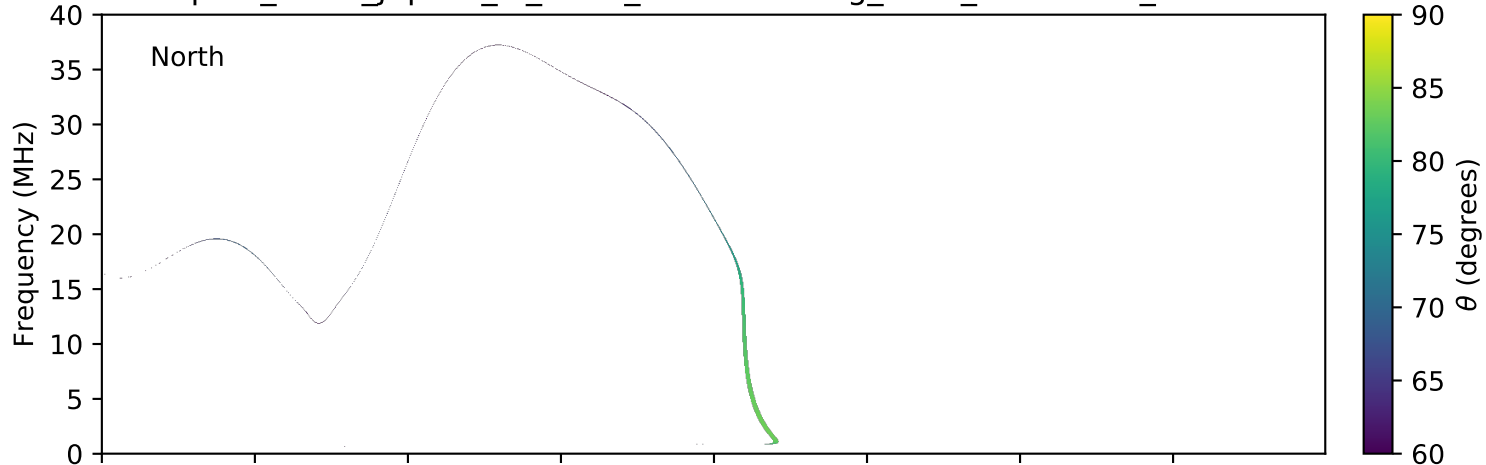
expres_earth_jupiter_io_isaac_lossc-wid1deg_3kev_20150627_v01.cdf
