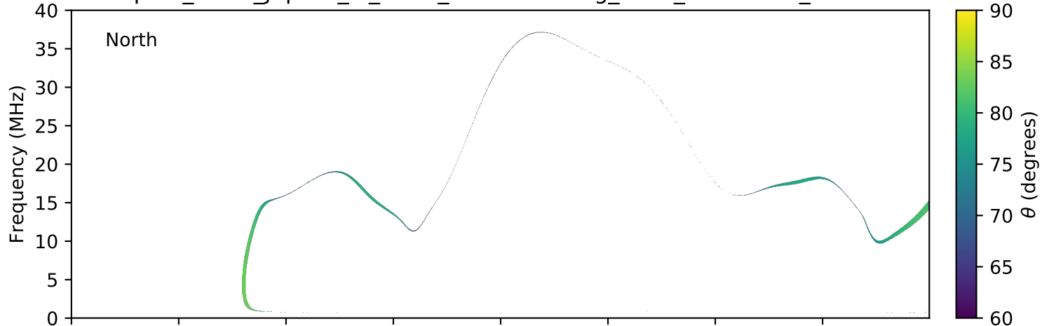
expres_earth_jupiter_io_isaac_lossc-wid1deg_3kev_20150623_v01.cdf
