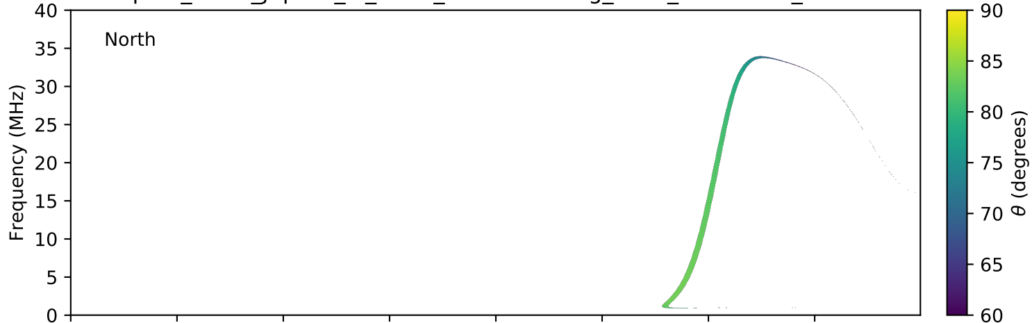
expres_earth_jupiter_io_isaac_lossc-wid1deg_3kev_20150619_v01.cdf
