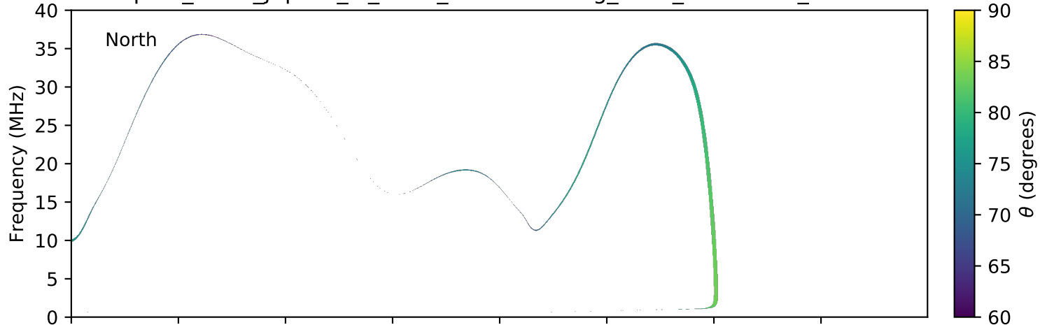
expres_earth_jupiter_io_isaac_lossc-wid1deg_3kev_20150618_v01.cdf
