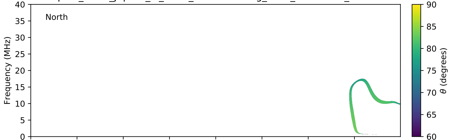
expres_earth_jupiter_io_isaac_lossc-wid1deg_3kev_20150617_v01.cdf
