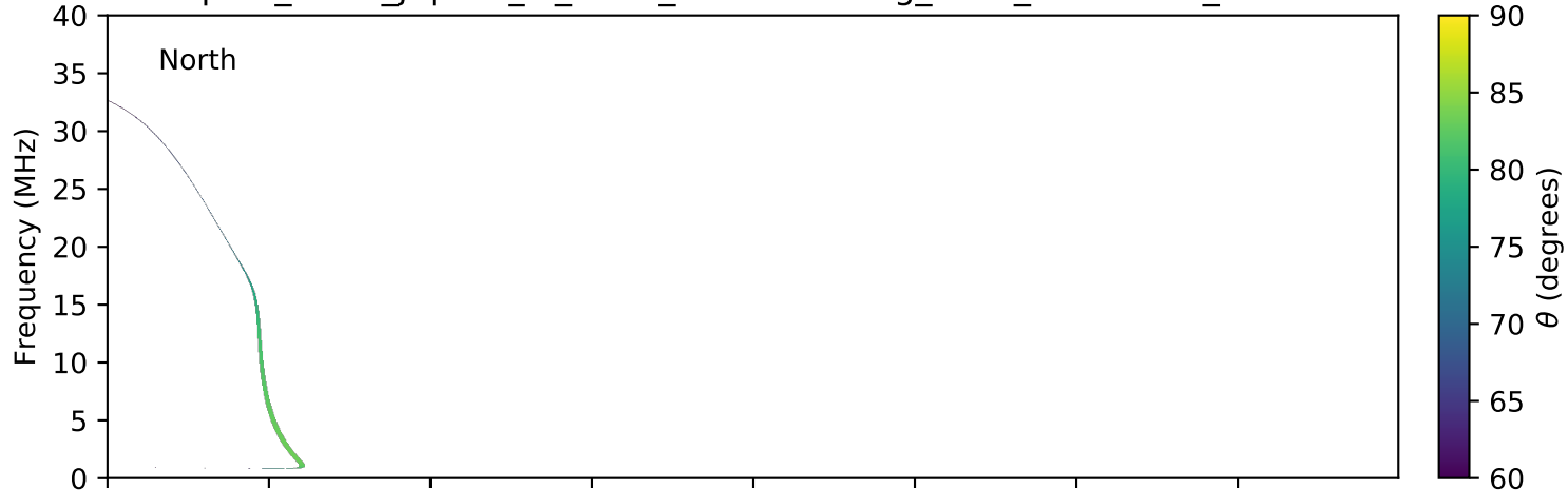
expres_earth_jupiter_io_isaac_lossc-wid1deg_3kev_20150615_v01.cdf
