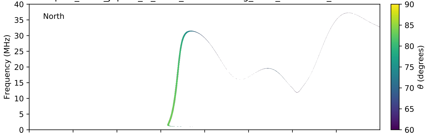
expres_earth_jupiter_io_isaac_lossc-wid1deg_3kev_20150614_v01.cdf
