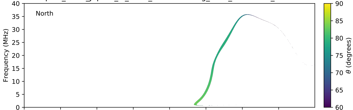
expres_earth_jupiter_io_isaac_lossc-wid1deg_3kev_20150612_v01.cdf
