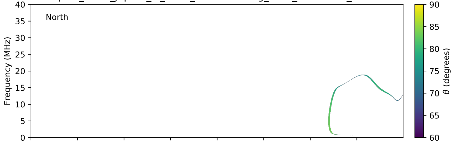
expres_earth_jupiter_io_isaac_lossc-wid1deg_3kev_20150610_v01.cdf
