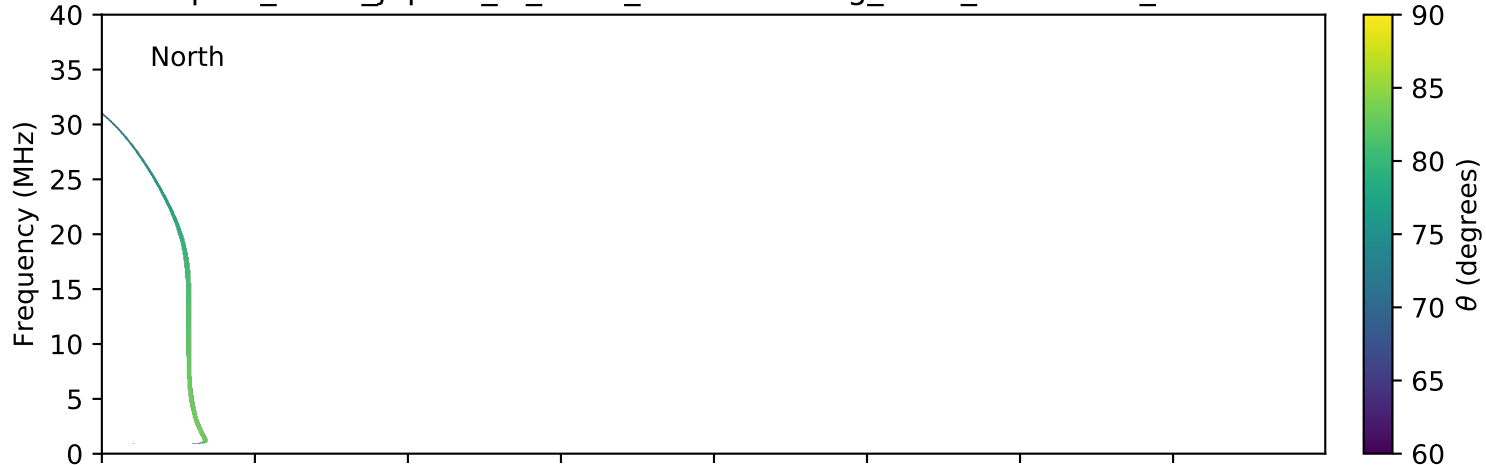
expres_earth_jupiter_io_isaac_lossc-wid1deg_3kev_20150608_v01.cdf
