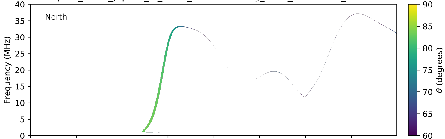
expres_earth_jupiter_io_isaac_lossc-wid1deg_3kev_20150607_v01.cdf
