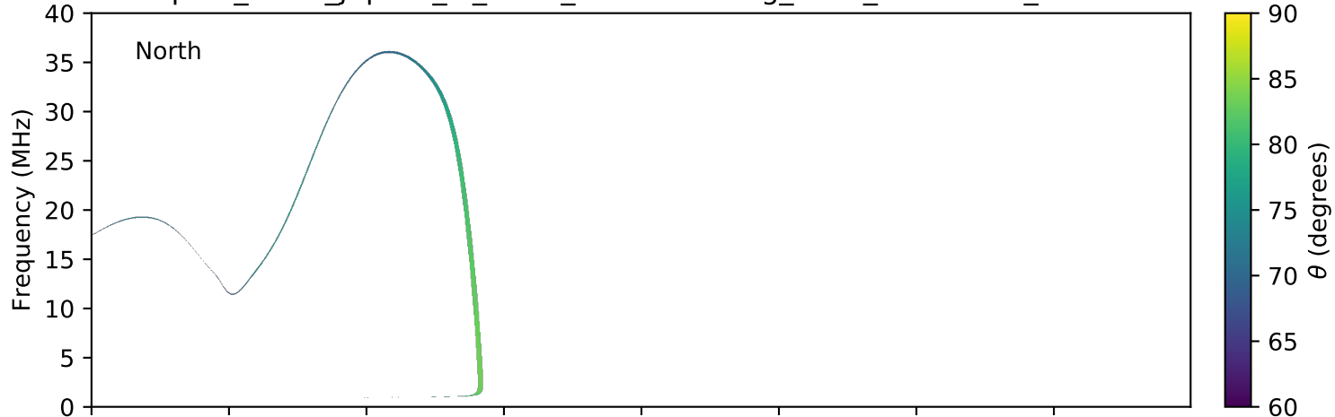
expres_earth_jupiter_io_isaac_lossc-wid1deg_3kev_20150606_v01.cdf
