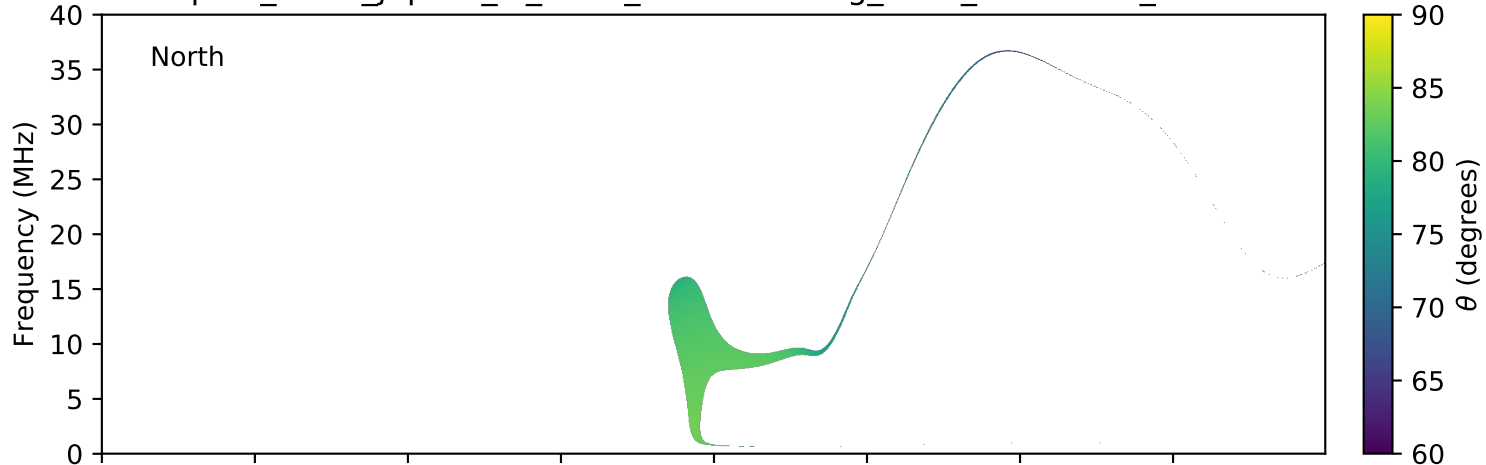
expres_earth_jupiter_io_isaac_lossc-wid1deg_3kev_20150605_v01.cdf
