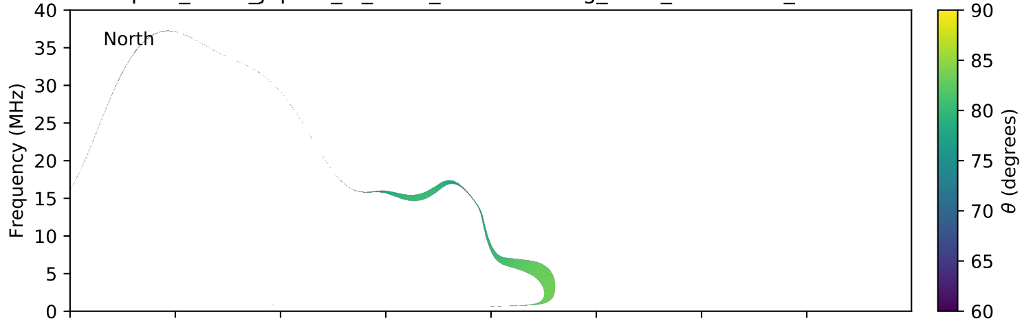
expres_earth_jupiter_io_isaac_lossc-wid1deg_3kev_20150604_v01.cdf
