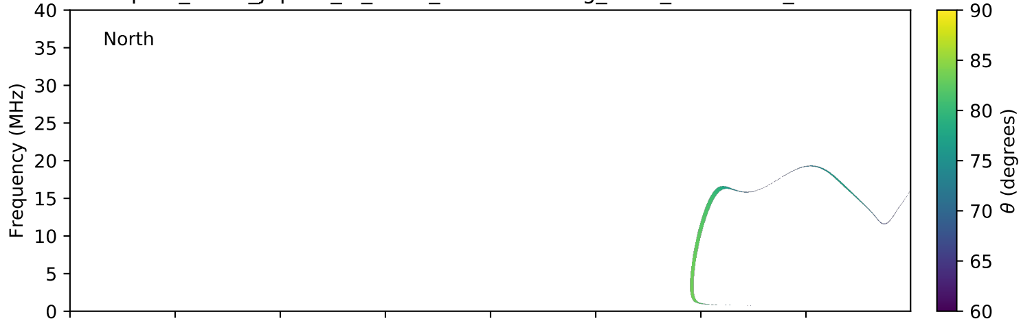
expres_earth_jupiter_io_isaac_lossc-wid1deg_3kev_20150603_v01.cdf
