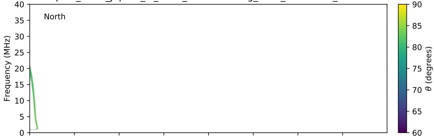
expres_earth_jupiter_io_isaac_lossc-wid1deg_3kev_20150601_v01.cdf
