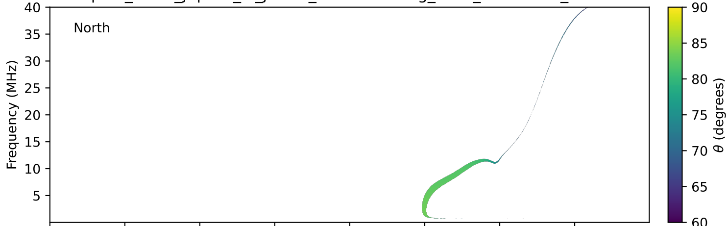
expres_earth_jupiter_io_jrm33_lossc-wid1deg_3kev_20150504_v11.cdf
