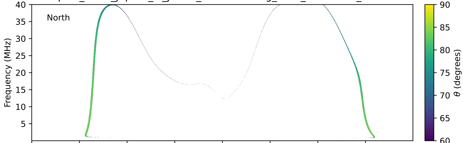
expres_earth_jupiter_io_jrm33_lossc-wid1deg_3kev_20150501_v11.cdf
