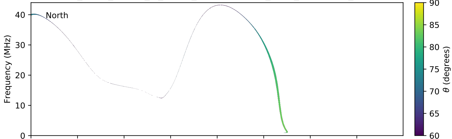
expres_earth_jupiter_io_jrm09_lossc-wid1deg_3kev_20150526_v01.cdf
