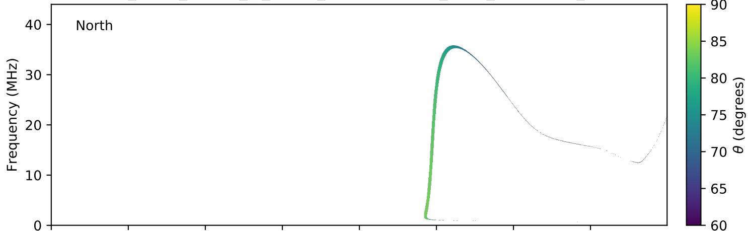
expres_earth_jupiter_io_jrm09_lossc-wid1deg_3kev_20150520_v01.cdf
