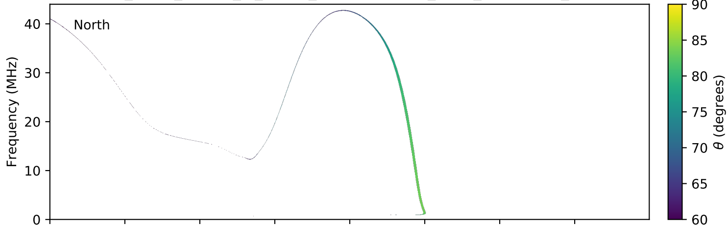
expres_earth_jupiter_io_jrm09_lossc-wid1deg_3kev_20150519_v01.cdf
