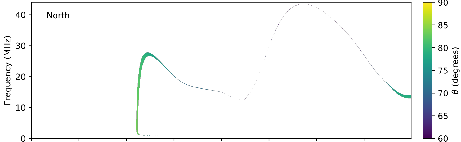
expres_earth_jupiter_io_jrm09_lossc-wid1deg_3kev_20150515_v01.cdf
