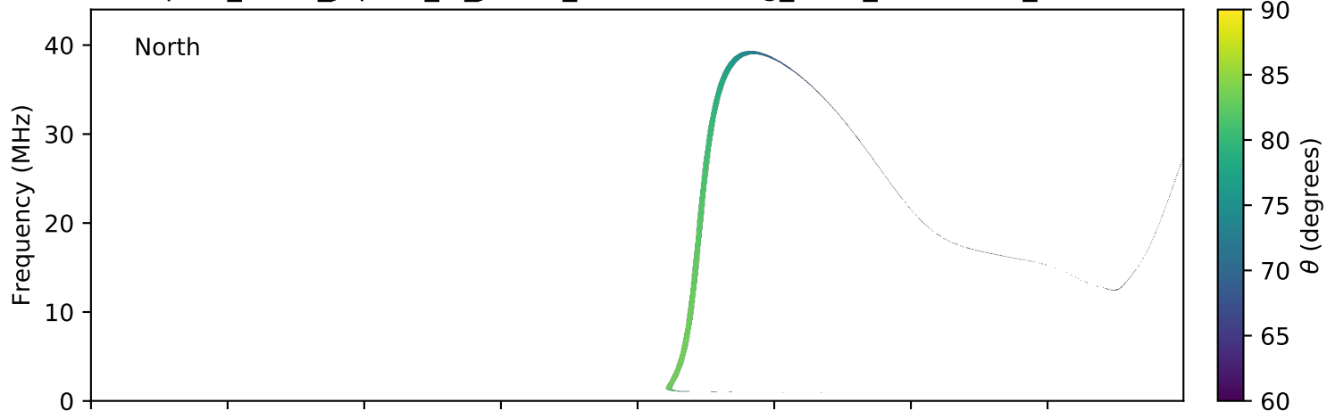
expres_earth_jupiter_io_jrm09_lossc-wid1deg_3kev_20150513_v01.cdf
